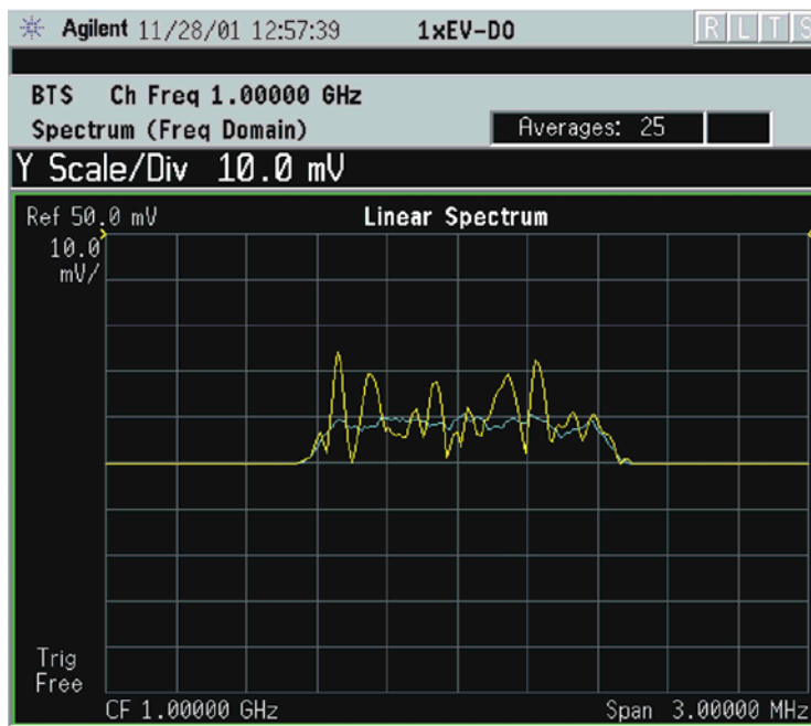
Figure 2-48 Spectrum Measurement - Linear Spectrum View (for E4406A)
