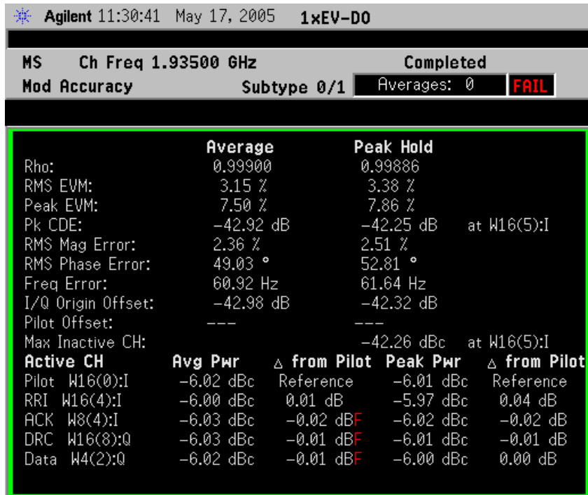
Figure 2-32 Reverse Link Modulation Accuracy Measurement Result - Peak/Average Metrics View
