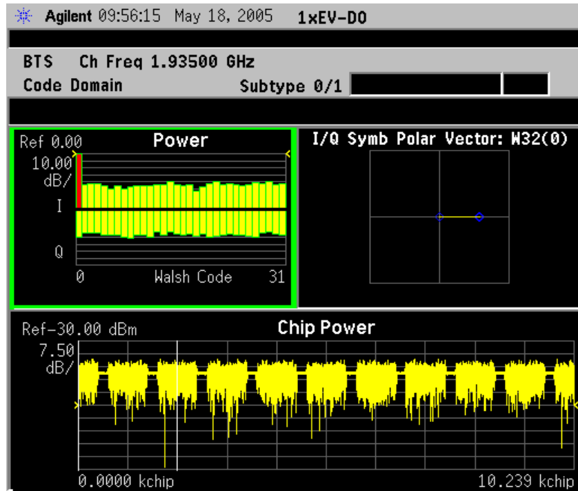
Figure 2-8 Forward Link Code Domain Measurement Result - I/Q Polar and Power Graph View- Subtype 0/1
