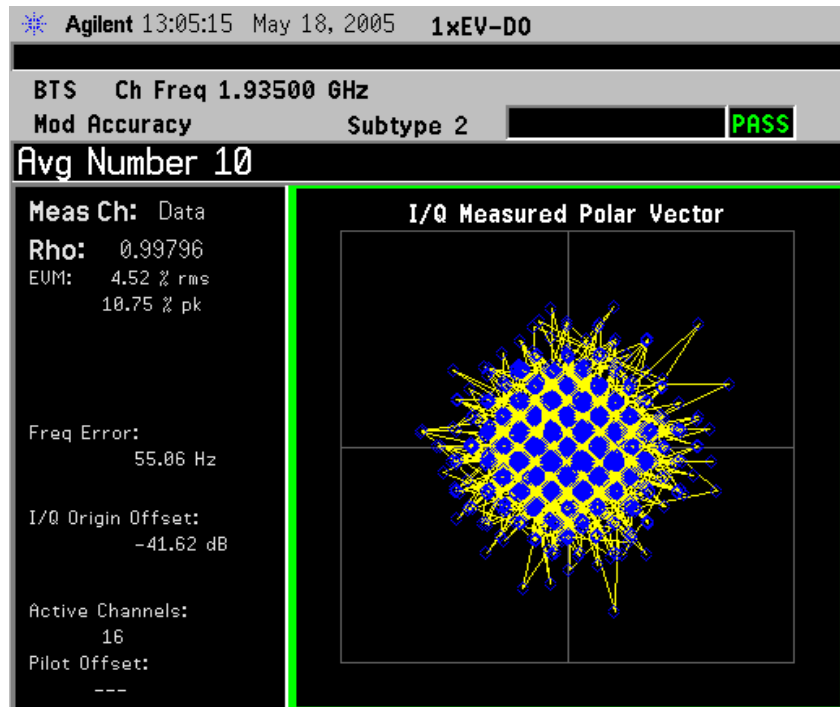
Figure 2-25 Forward Link Modulation Accuracy Measurement Result - I/Q Measured Polar Vector View
