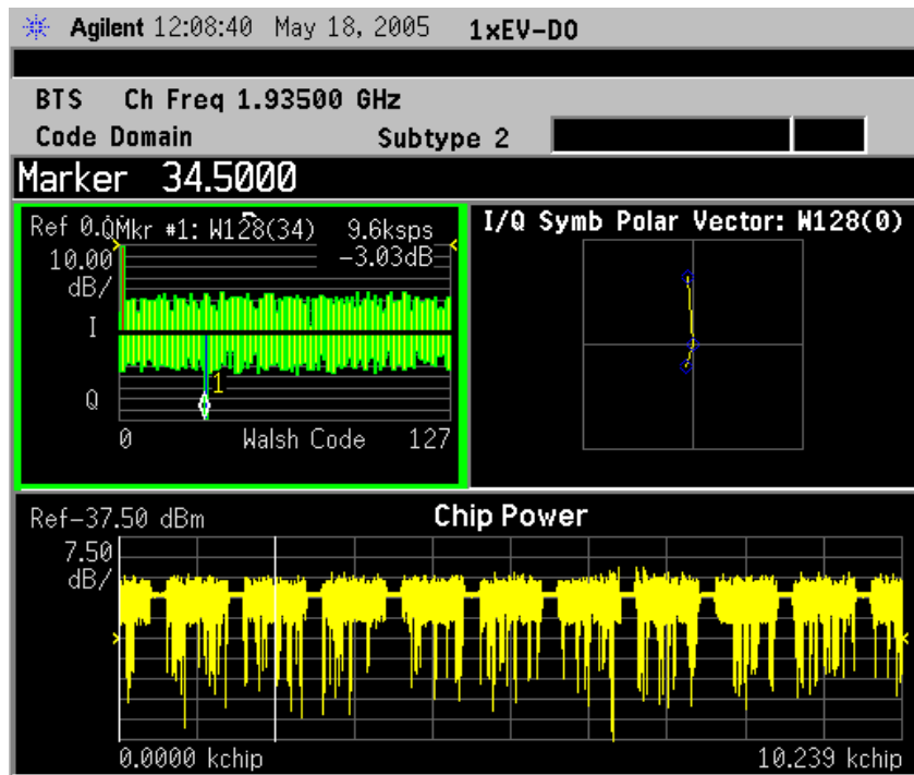
Figure 2-9 Forward Link Code Domain Measurement Result - I/Q Polar and Power Graph View - Subtype 2
