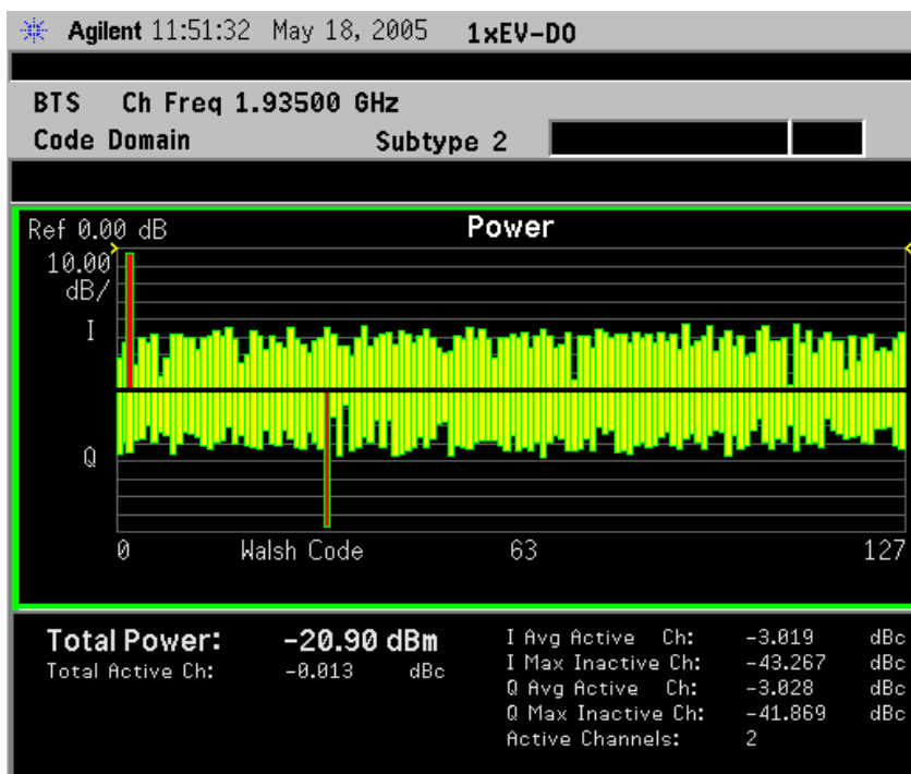
Figure 2-7 Forward Link Code Domain Measurement Result - Power Graph (Default) View - Subtype 2
