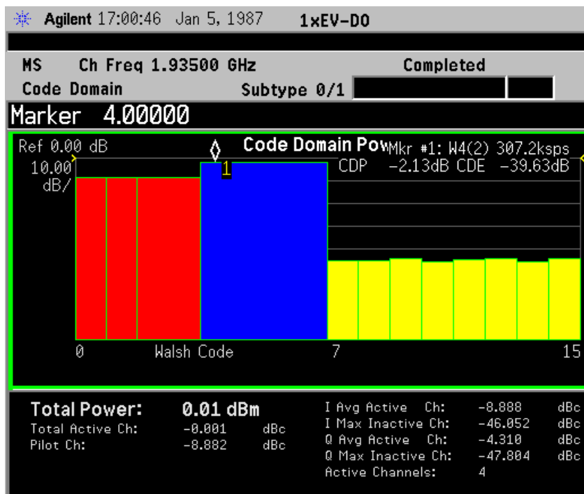
Figure 2-16 Reverse Code Domain Measurement Result - Code Domain Power Graph View with Bit Reverse Display (I/Q Combined)
