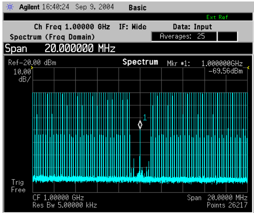
Figure 2-53 Spectrum Measurement - Spectrum View with Opt. 122– 80 MHz Bandwidth Digitizer Hardware
