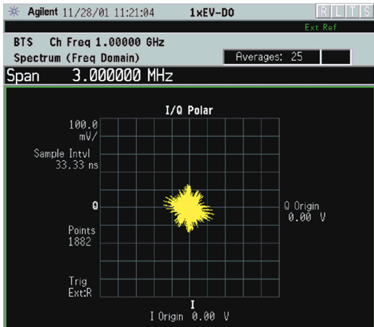
Figure 2-50 Spectrum Measurement - I/Q Polar View (for E4406A)
