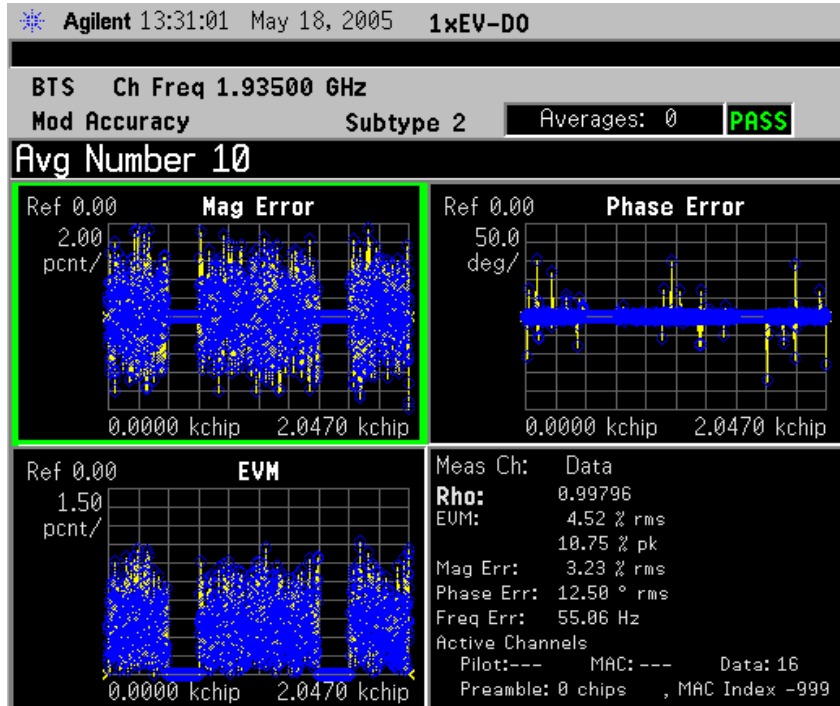
Figure 2-27 Forward Link Modulation Accuracy Measurement Result - I/Q Error Quad View
