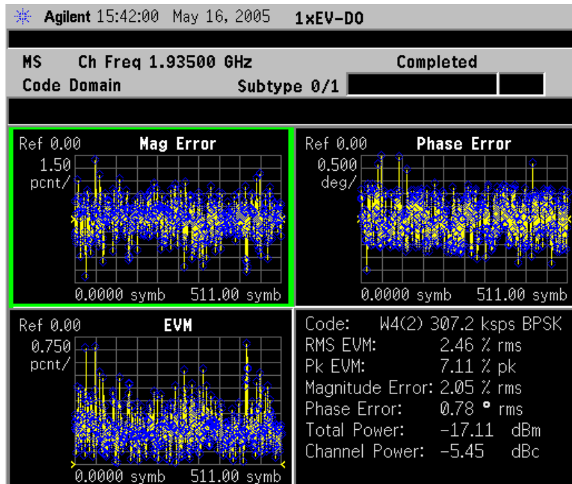
Figure 2-18 Reverse Link Code Domain Measurement - I/Q Error (Quad View)
