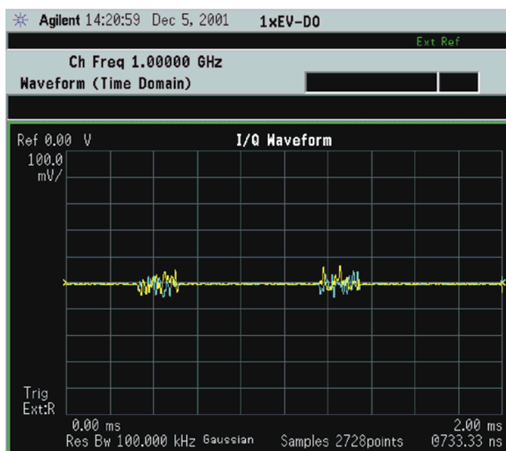
Figure 2-61 Waveform Measurement - I/Q Waveform View
