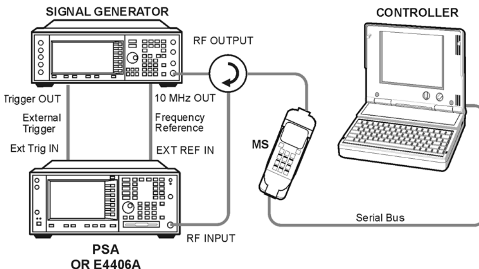
Figure 2-11 Power Control Measurement System
