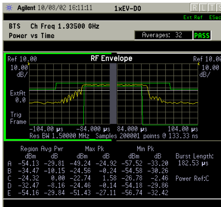
Figure 2-41 Power Vs. Time Measurement Result - Rise and Fall View
