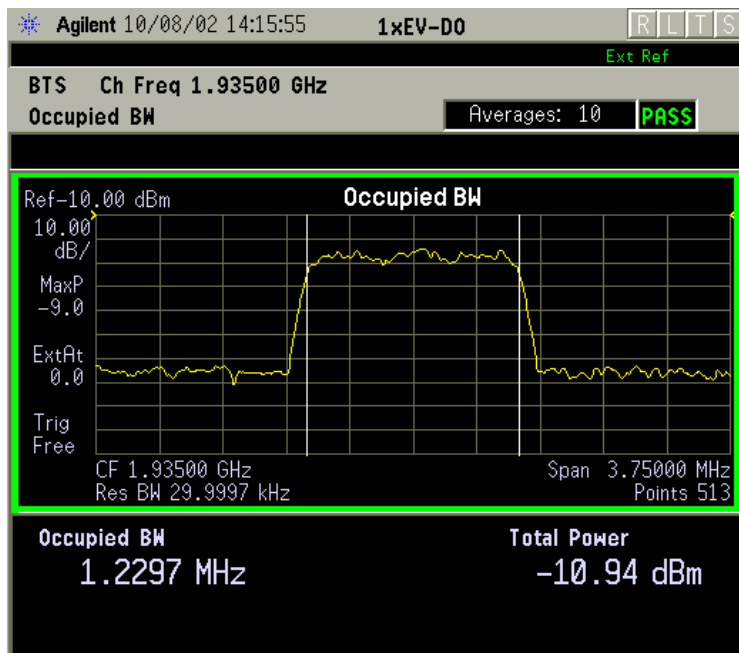
Figure 2-36 Occupied Bandwidth Measurement Result
