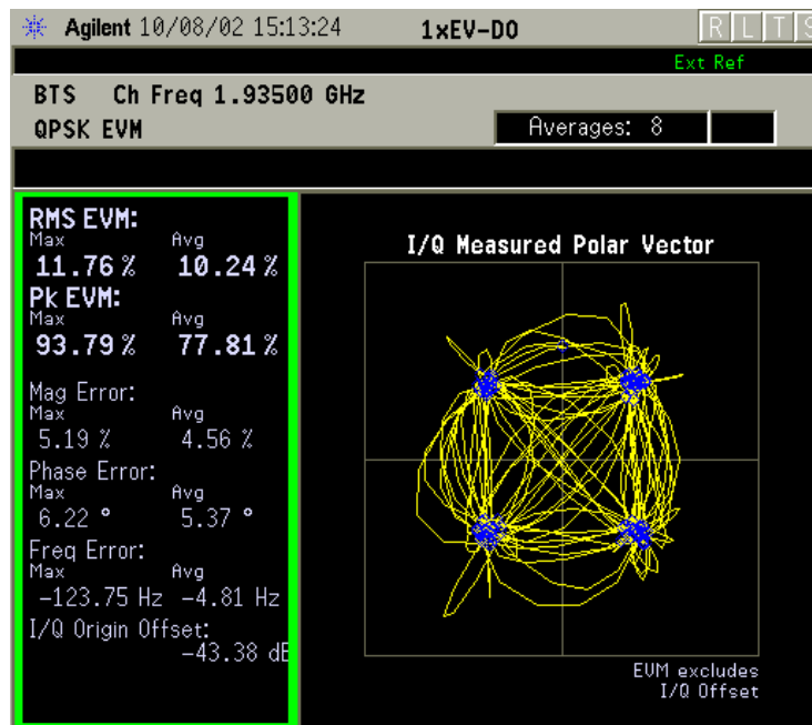
QPSK EVM Measurement Result - Polar Vector (Default) View
