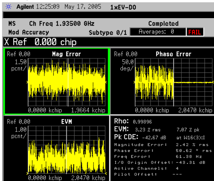
Figure 2-33 Reverse Link Modulation Accuracy Measurement Result - I/Q Error Quad View
