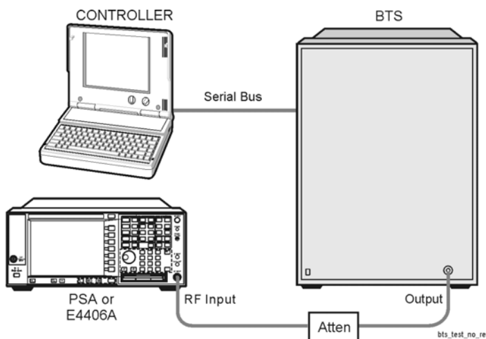
Power Statistics (CCDF) Measurement System
