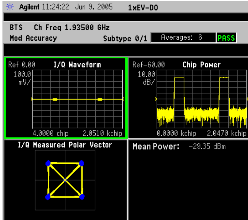
Figure 2-28 Forward Link Modulation Accuracy Measurement Result - I/Q Measured (Quad View)
