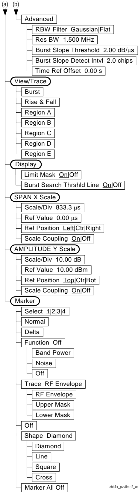
Figure 6-18 Power vs. Time Measurement Key Flow (2 of 2)
