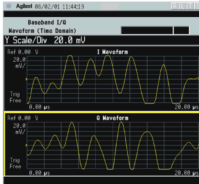
Figure 3-35 Waveform Measurement - I and Q Waveform View
