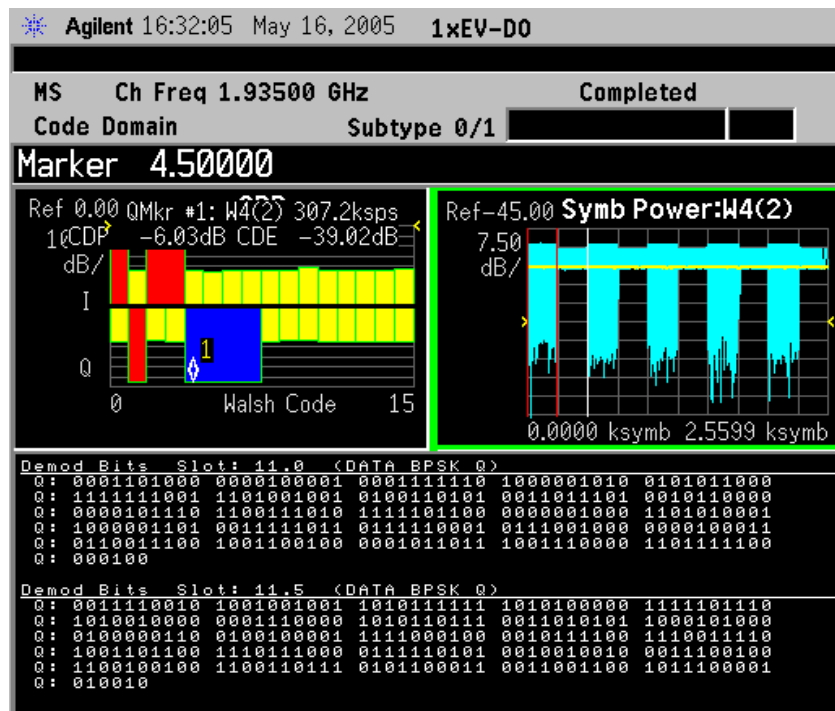
Figure 2-20 Reverse Link Code Domain Measurement - Demod Bits View
