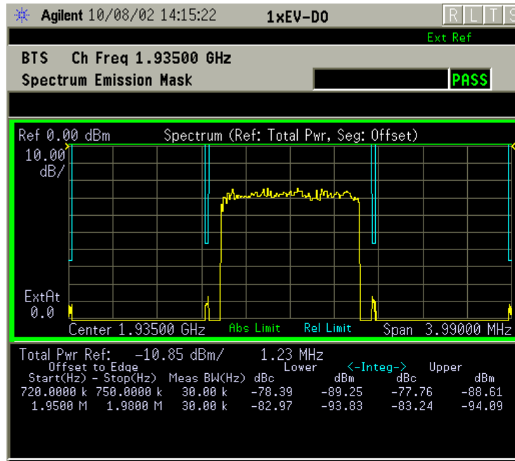
Figure 2-58 Spectrum Emission Mask Measurement Result - ACP View
