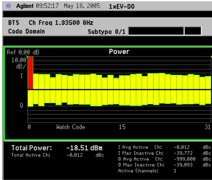
Figure 2-6 Forward Link Code Domain Measurement Result - Power Graph (Default) View- Subtype 0/1
