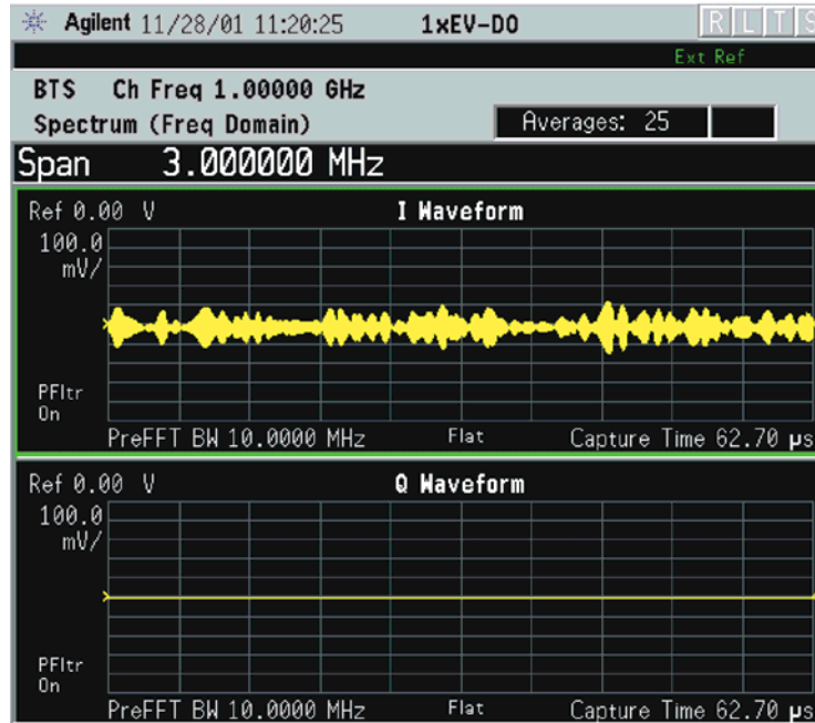
Figure 2-49 Spectrum Measurement - I and Q Waveform View (for E4406A)
