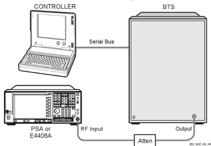
Figure 2-35 Occupied Bandwidth Measurement System
