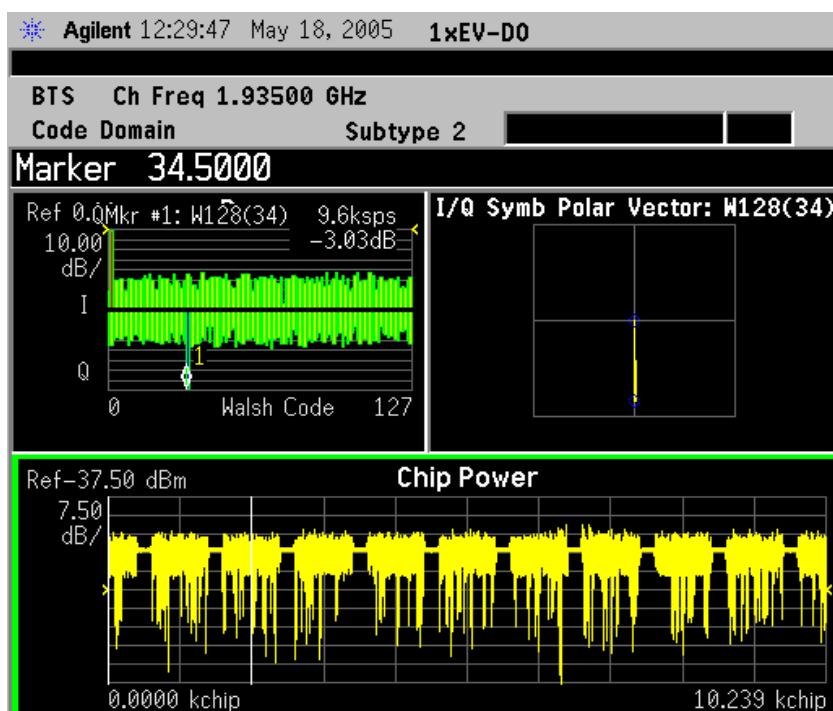
Figure 2-10 Forward Link Code Domain Measurement Result - I/Q Polar and Power Graph View - Subtype 2 with W128(34) Despread
