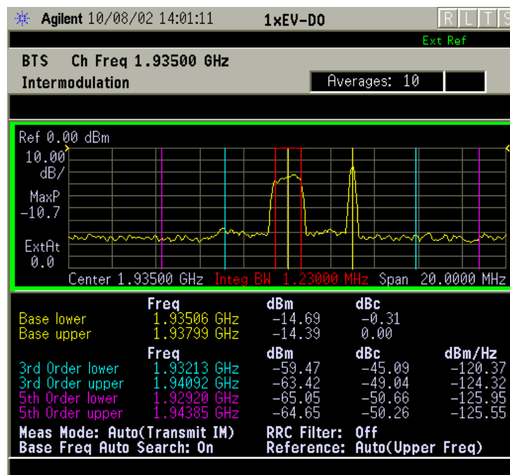
Figure 2-23 Intermodulation Measurement Result
