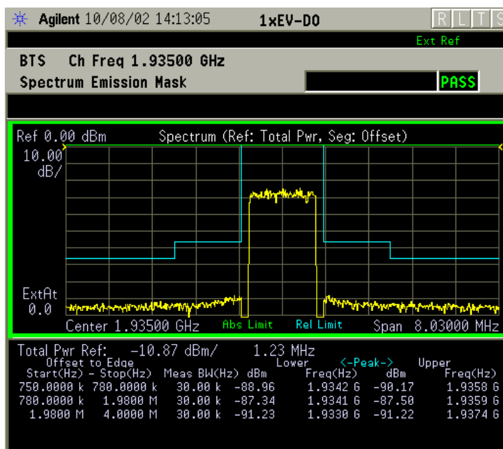
Figure 2-56 Spectrum Emission Mask Measurement Result - Offset (Default) View
