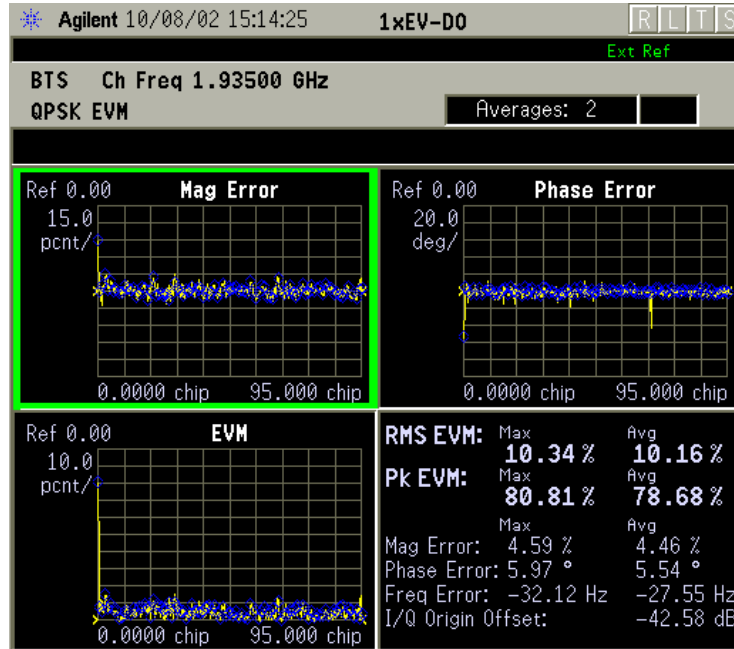
Figure 2-45 QPSK EVM Measurement Result - I/Q Error Quad View
