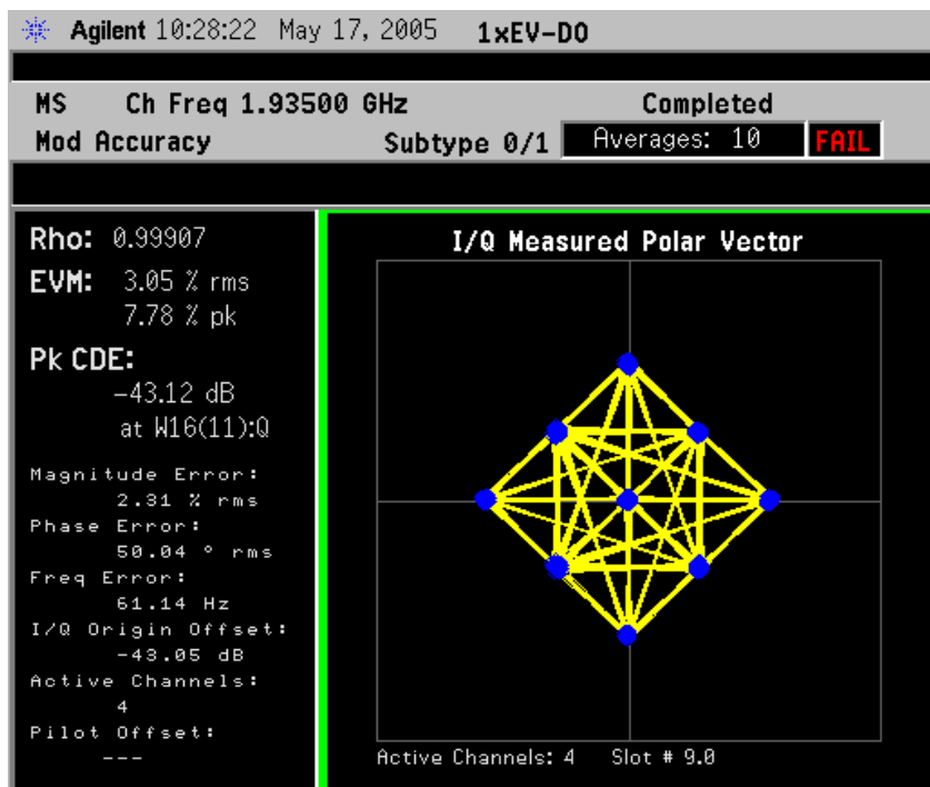
Figure 2-31 Reverse Link Modulation Accuracy Measurement Result - Measured Polar Vector Graph (Default) View
