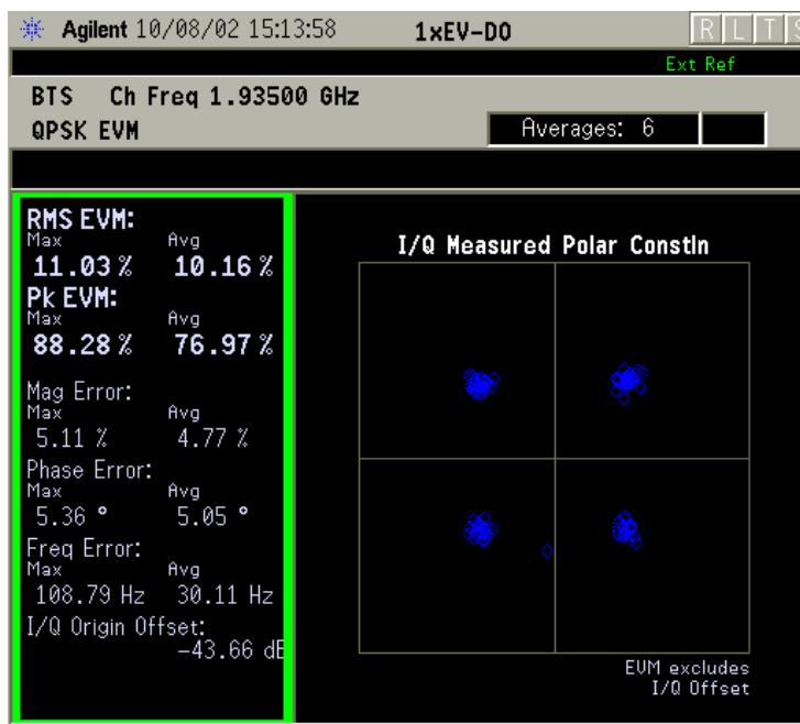
Figure 2-44 QPSK EVM Measurement Result - Polar Constellation View
