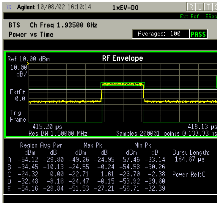
Figure 2-40 Power Vs. Time Measurement Result - RF Envelope (Default) View
