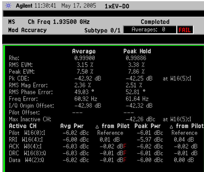
Figure 3-16 Modulation Accuracy Measurement - Peak/Avg Metrics View
