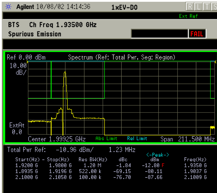
Figure 2-57 Spectrum Emission Mask Measurement Result - Region View
