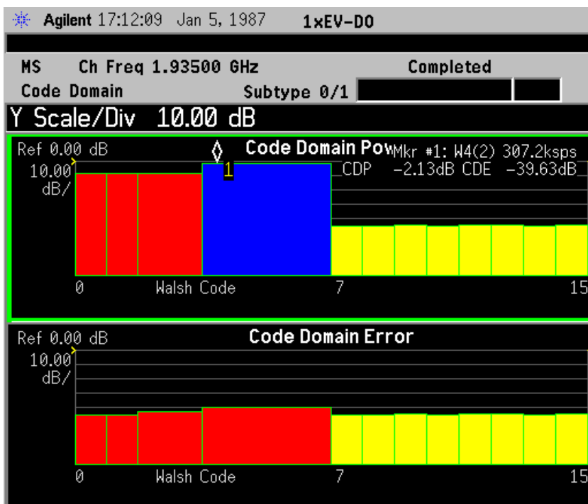
Figure 2-17 Reverse Link Code Domain Measurement - CDP & CDE View
