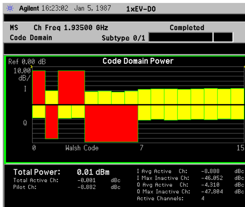
Figure 2-14 Reverse Code Domain Measurement Result - Code Domain Power Graph View with Bit Reverse Display
