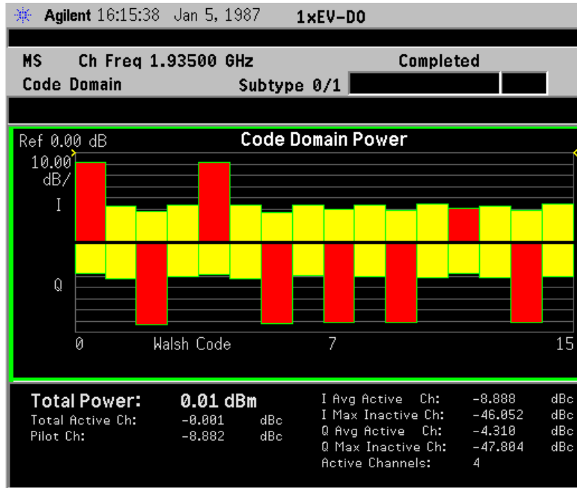
Figure 2-12 Reverse Code Domain Measurement Result - Code Domain Power Graph (Default) View
